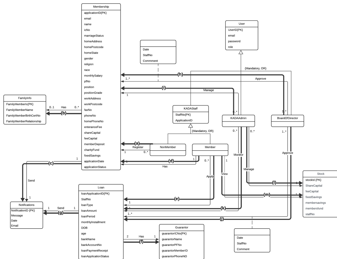
Figure 3.2: Verified ERD
